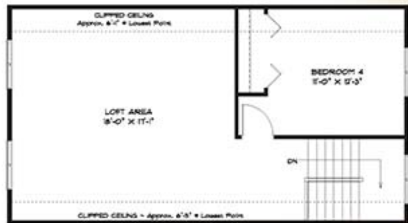
OPT LOFT A 580 SQ. FT
