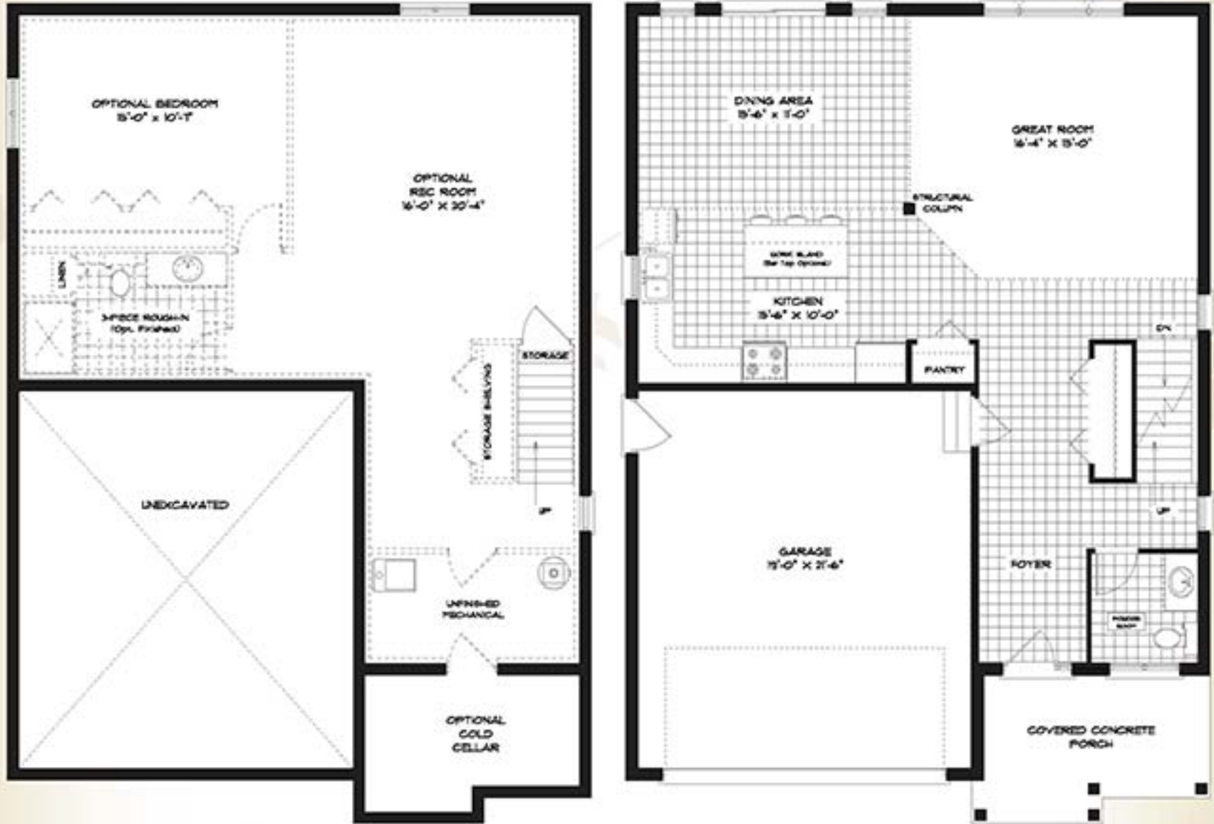
BASEMENT PLAN
