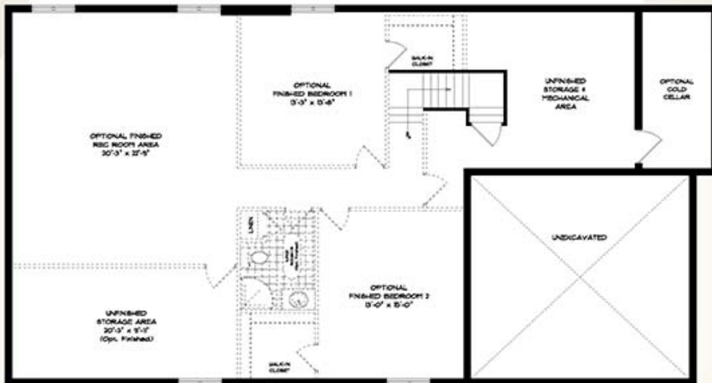
BASEMENT PLAN
