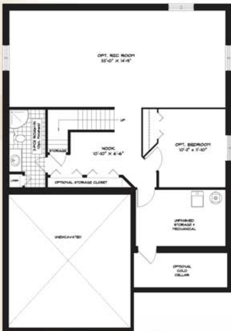
BASEMENT PLAN
