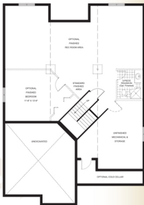
BASEMENT PLAN
